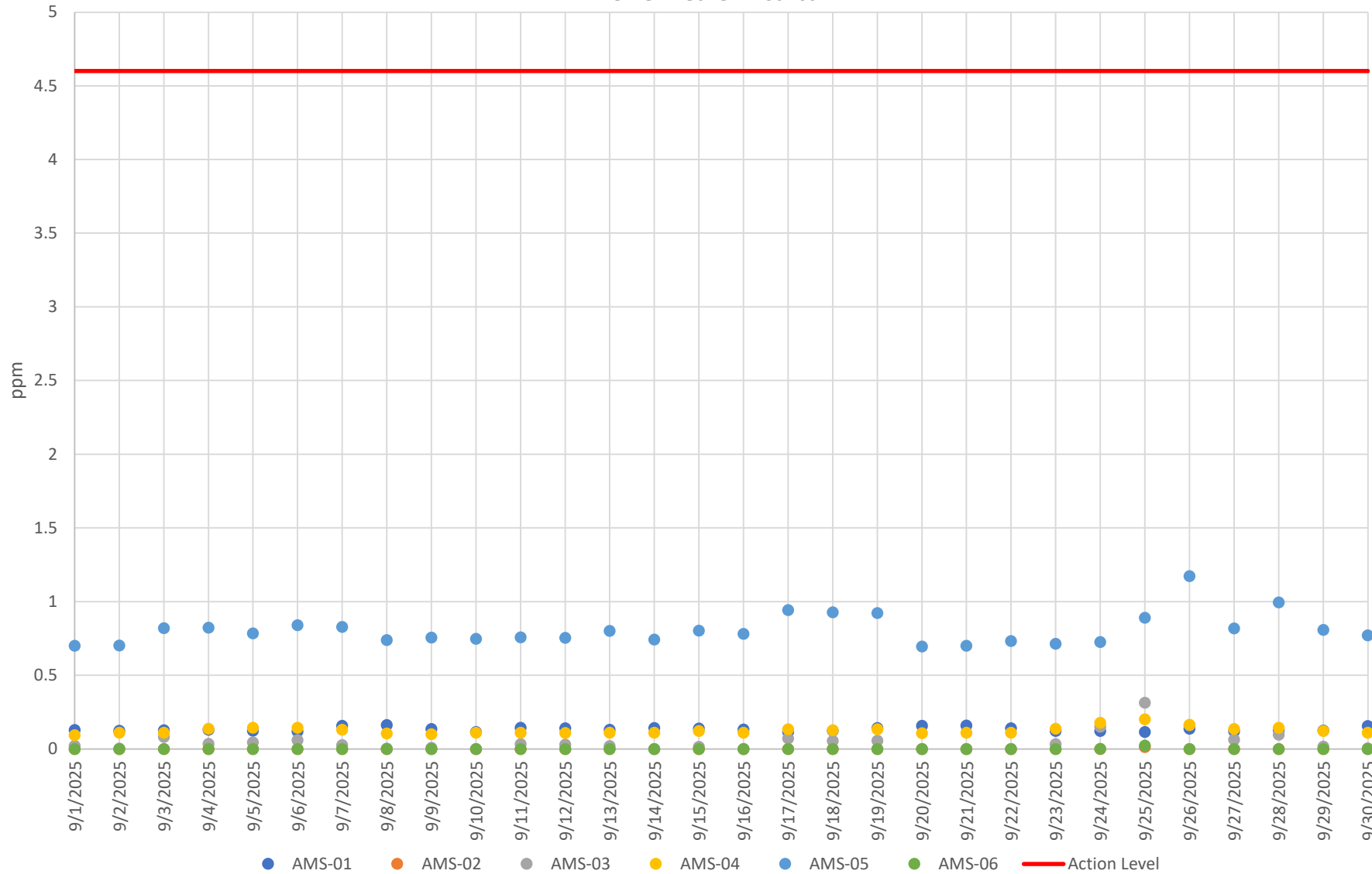
Figure 3.a - VOC Concentration 8-Hour Averages Industrial Campus Sep. 1, 2025 – Sep. 30, 2025 The Bellwether District
