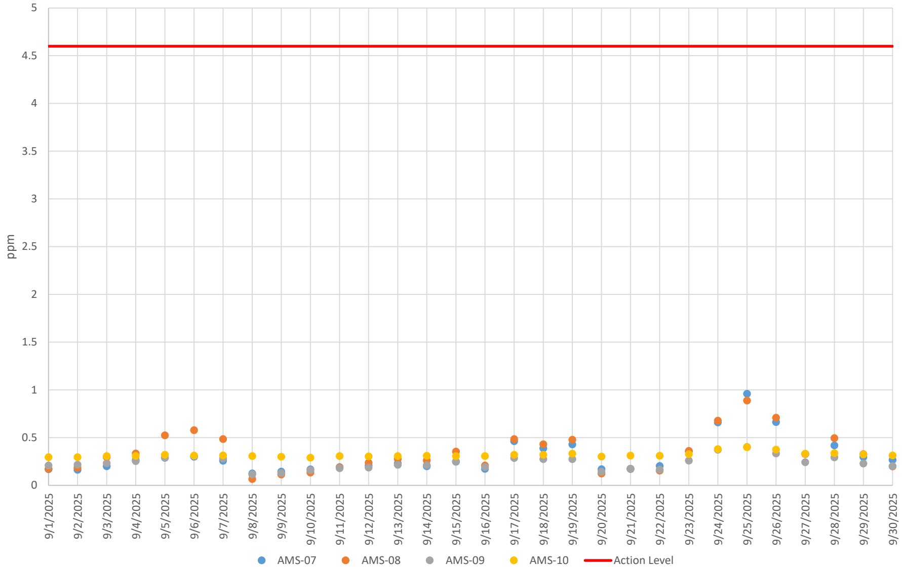
Figure 3.b - VOC Concentration 8-Hour Averages Innovation Campus Sep. 1, 2025 – Sep. 30, 2025 The Bellwether District
