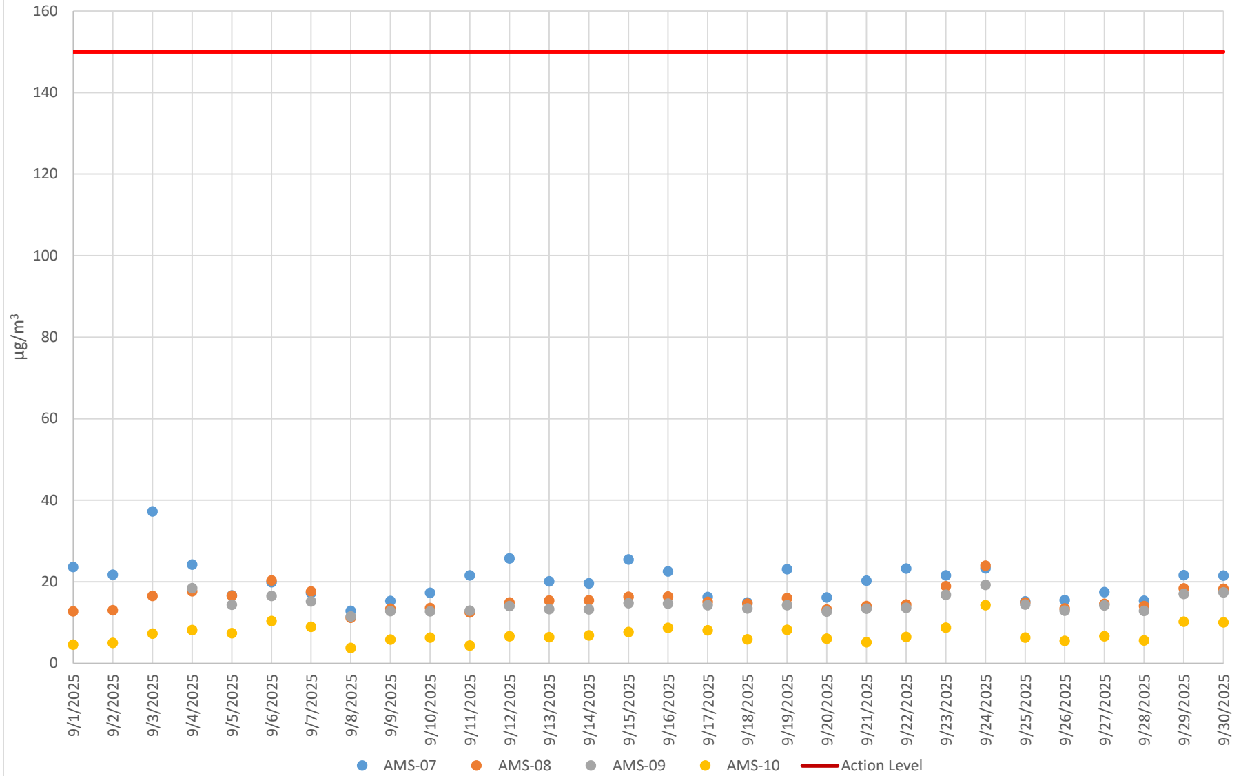
Figure 2.b - Dust Concentration 24-Hour Averages Innovation Campus Sep. 1, 2025 – Sep. 30, 2025 The Bellwether District
