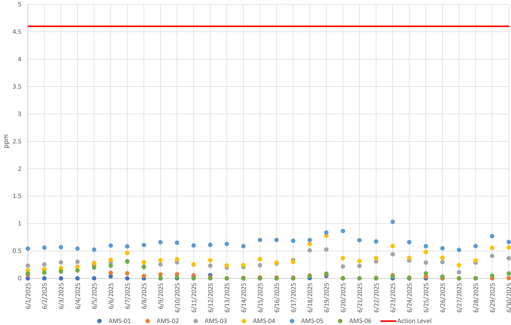
Figure 3.a - VOC Concentration 8-Hour Averages Industrial Campus Jun. 1, 2025 – Jun. 30, 2025 The Bellwether District
