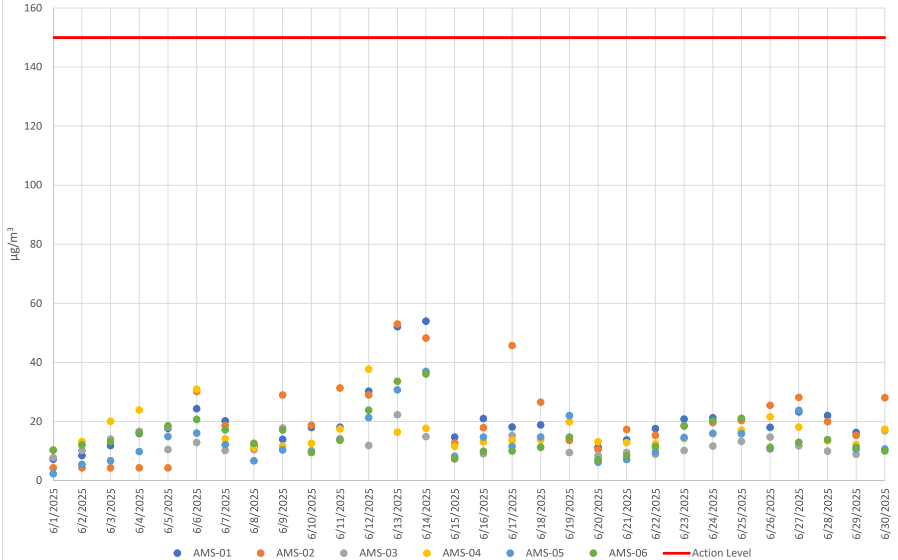
Figure 2.a - Dust Concentration 24-Hour Averages Industrial Campus Jun. 1, 2025 – Jun. 30, 2025 The Bellwether District
