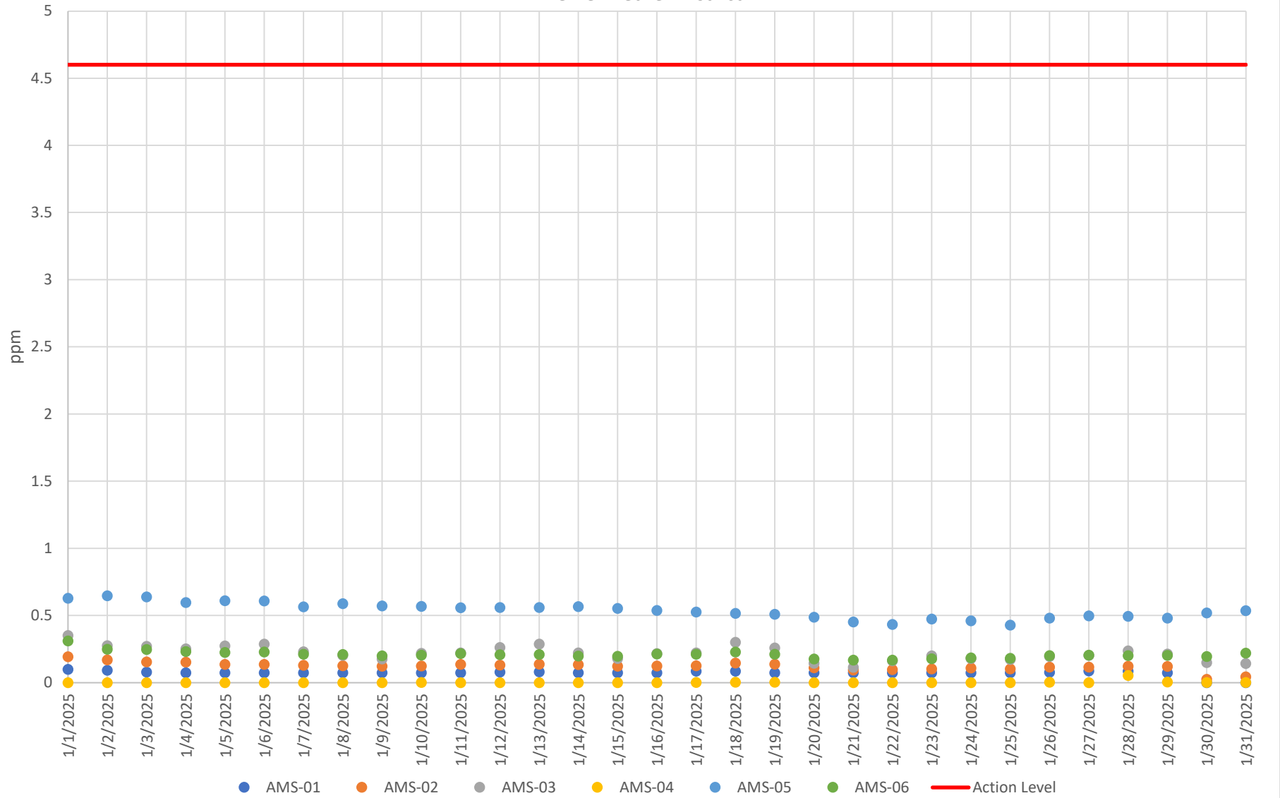
Figure 3.a - VOC Concentration 8-Hour Averages Industrial Campus Jan. 1, 2025 – Jan. 31, 2025 The Bellwether District
