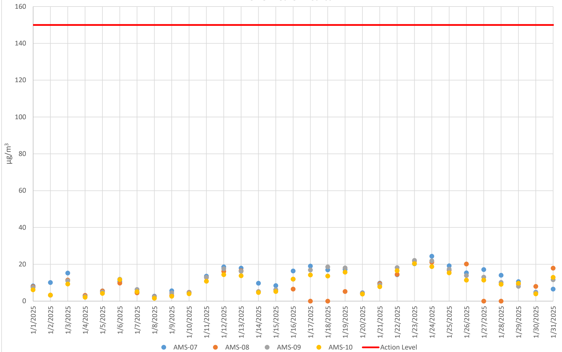
Figure 2.b - Dust Concentration 24-Hour Averages Innovation Campus Jan. 1, 2025 – Jan. 31, 2025 The Bellwether District
