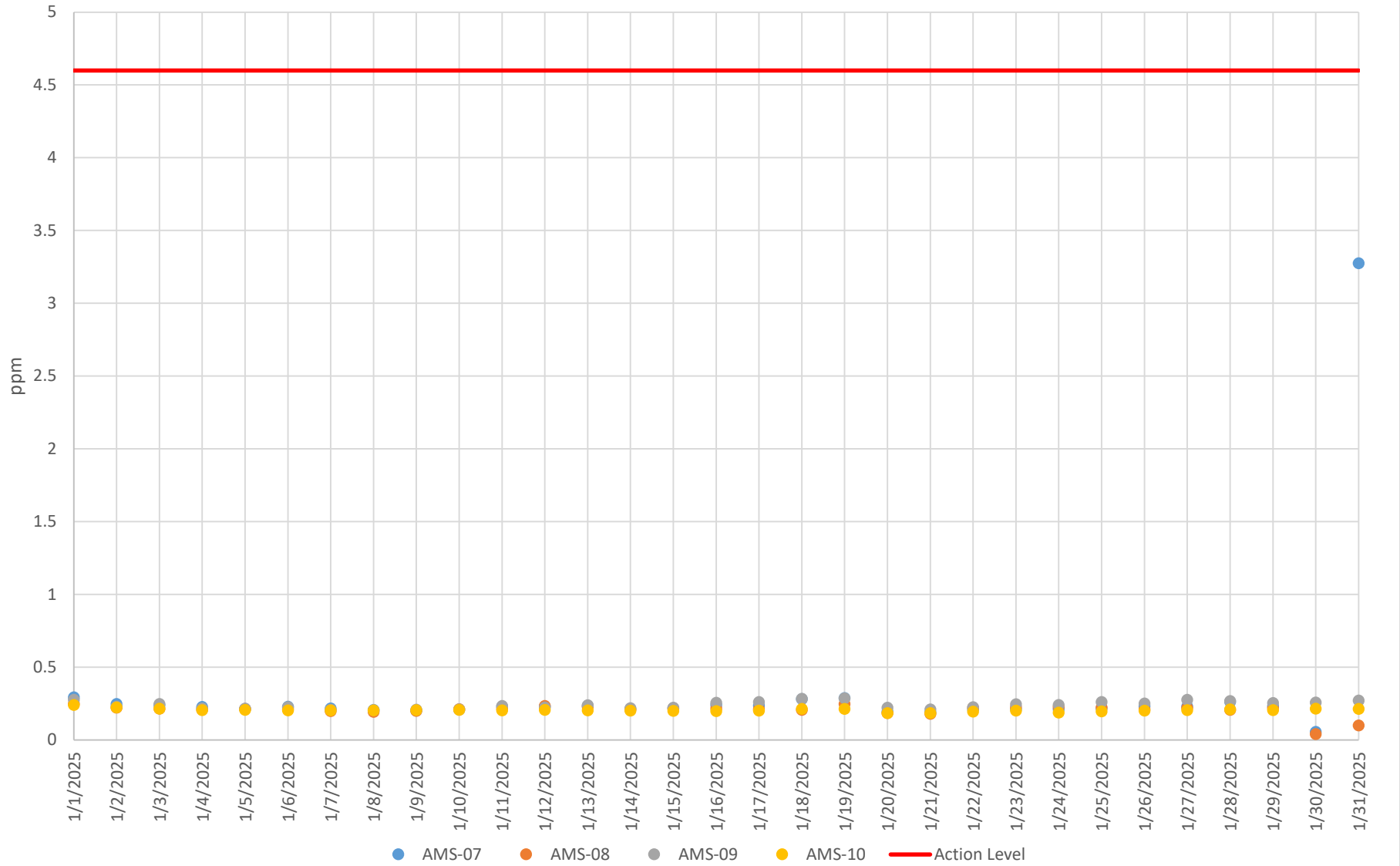
Figure 3.b - VOC Concentration 8-Hour Averages Innovation Campus Jan. 1, 2025 – Jan. 31, 2025 The Bellwether District
