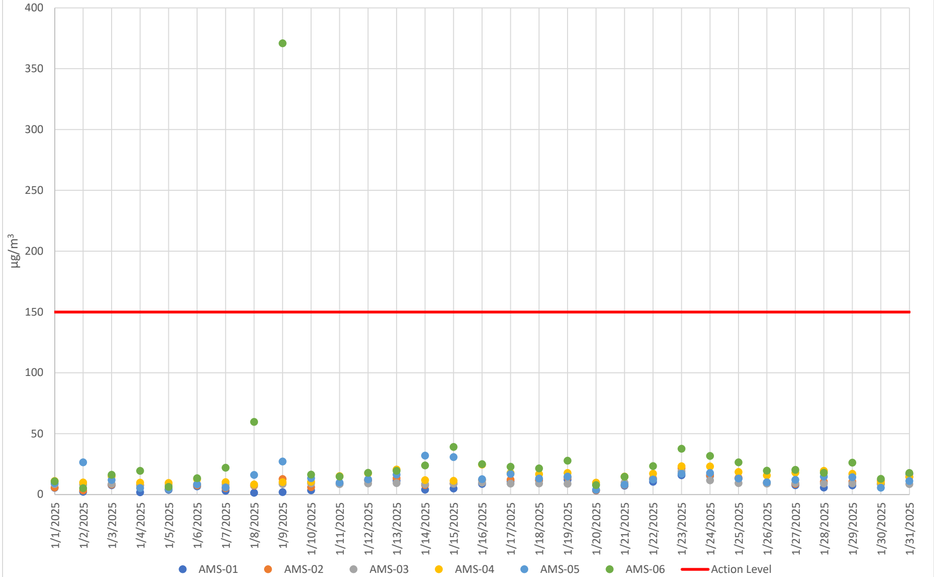
Figure 2.a - Dust Concentration 24-Hour Averages Industrial Campus Jan. 1, 2025 – Jan. 31, 2025 The Bellwether District
