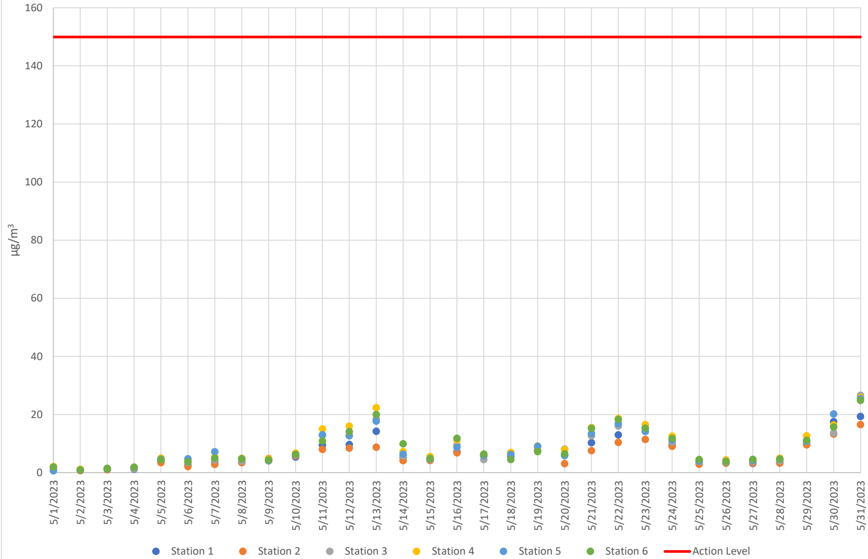
Figure 2 - Dust Concentration 24-Hour Averages May 1, 2023 – May 31, 2023 The Bellwether District
